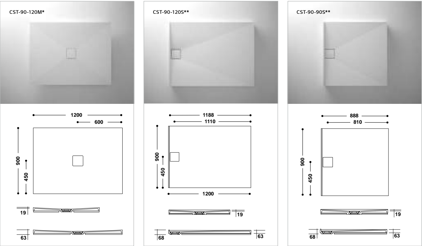
* Middle Drainhole
